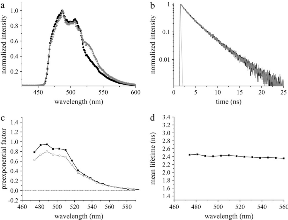
FIGURE 4 Fluorescence emission of Cerulean at 420 nm excitation in living COS-7 cells. (a) Comparison of fluorescence emission spectra of Cerulean alone (black) with coexpression of Cerulean and Citrine (shading). The fluorescence emission maximum for Cerulean was observed at 486 nm. A small Citrine component due to its high extinction coefficient was observed for the latter. (b) Fluorescence decay of Cerulean in the absence (black) and in the presence of Citrine (shading). IRF is shown in light shading. (c) DAS of Cerulean alone, which was unchanged in the presence of Citrine. Intensity decays were analyzed in 17 emission bands from 470 nm to 590 nm, and the preexponential factors of lifetimes \tau_1 (solid) and \tau_2 (shading) were plotted along the wavelength (Table 1). (d) Mean lifetimes of each emission band of Cerulean were plotted along the wavelength. Error bars are not shown due to their very small variability ( <0.05 ns).
